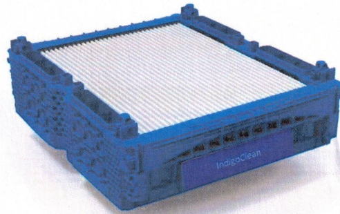
IndigoClean module with 6 m 2 filter area L x W x H [mm] = 700 x 655 x 160
